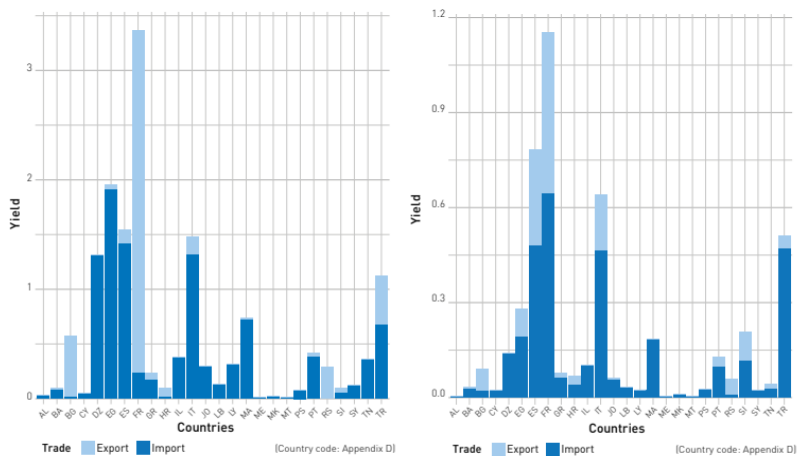
Figure 3.16 | Cereal trade patterns (average 2014-2017 values in tonnes x 10 7 ) in the Mediterranean countries: import (dark blue) and export (light blue) contribution for each Mediterranean country (identified by the ISO 3166-1 alpha-2 code) (FAO 2017).
